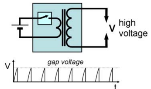
Figure 1: Principle example of a spark train generator.
